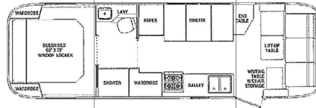
Model 30W Front Lounge Limited/Excelsa
