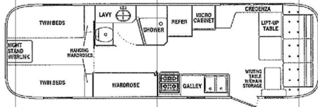
Model 31A Front Lounge Limited/Excelsa
