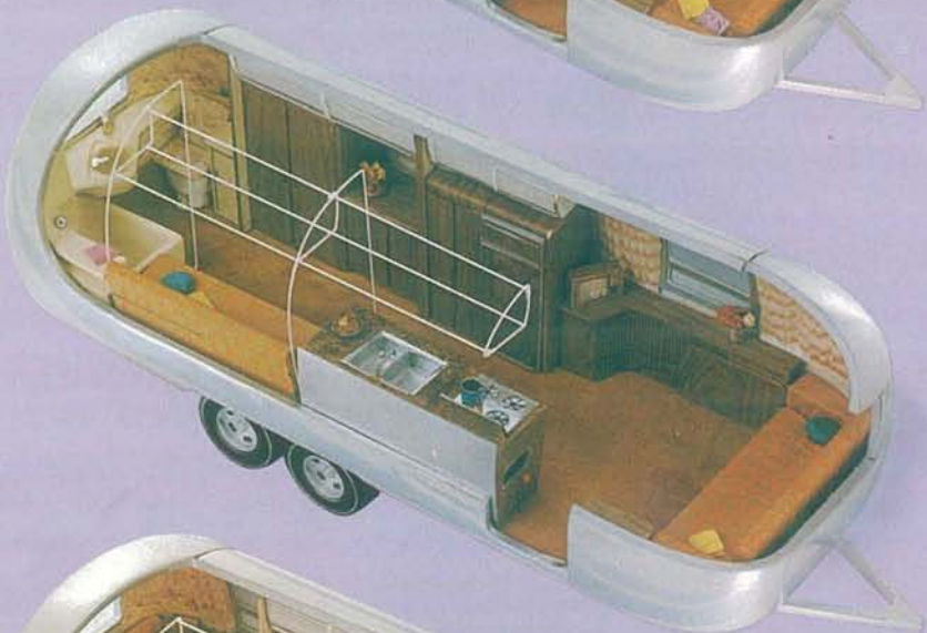
27 FT. OVERLANDER DOUBLE REAR BATH (International Land Yacht) Hitch Wt. 500 lbs. Total Wt. 4600 lbs.
