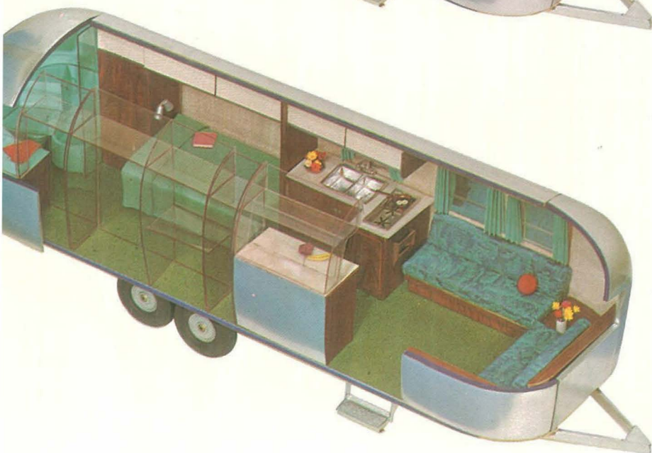
30 FT. SOVEREIGN DOUBLE Hitch Wt. 405 lbs. • Total Wt. 4650 lbs.
