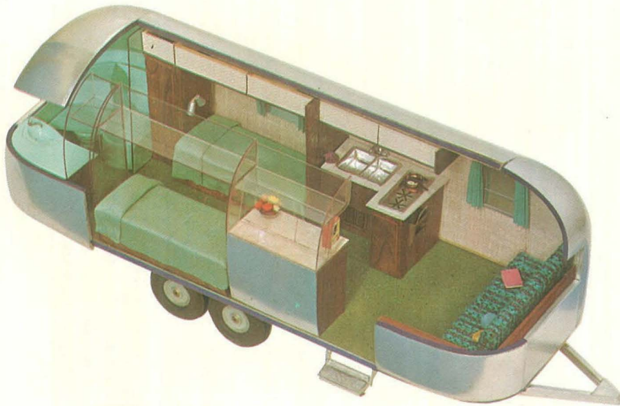
26 FT. OVERLANDER TWIN Hitch Wt. 450 lbs. • Total Wt. 4180 lbs.
