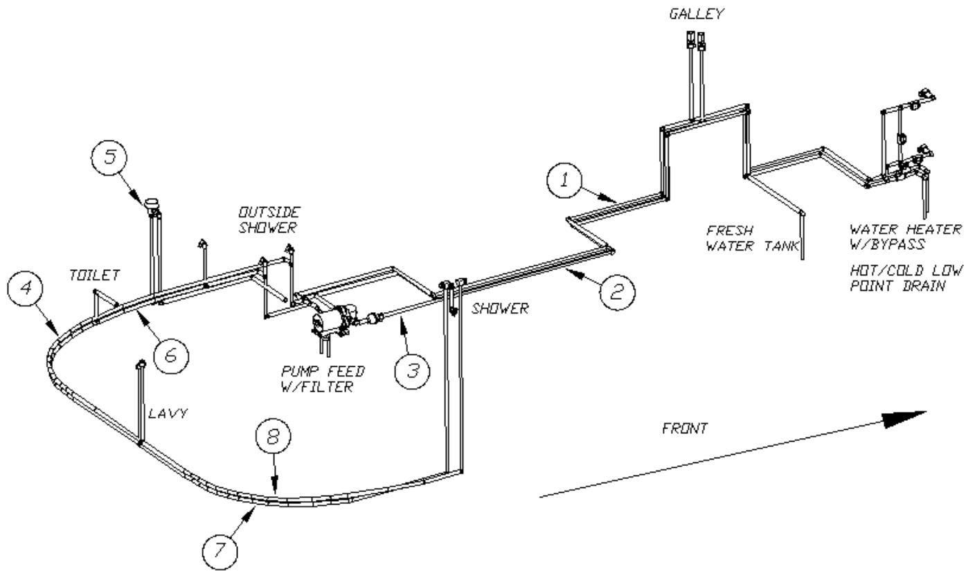
943692 Fresh Water Layout
