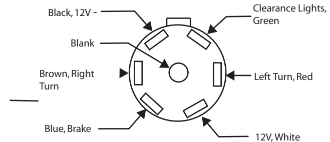
7-way Plug Diagram
